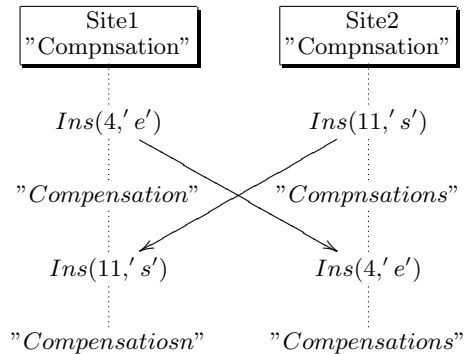
Figure 1: Divergence scenario
