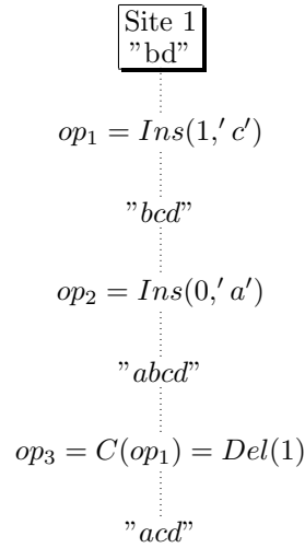
Figure 3: Naive compensation of a non-last executed operation
