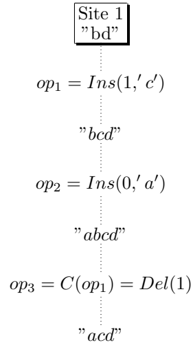
Figure 3: Naive compensation of a non-last executed operation
