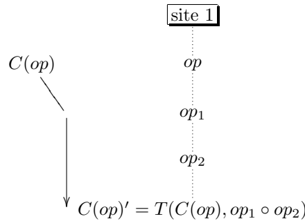
Figure 4: Algorithm of the compensation
