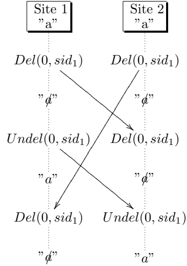
Figure 11: Violation of the property TP_1
