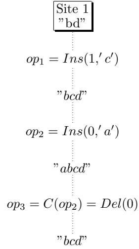
Figure 2: Compensation of a last executed operation
