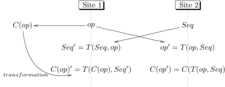
Figure 5: Respect of the compensation effect
