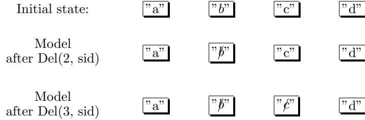
Figure 6: Model in the TTF approach.
