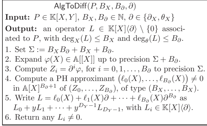
FIGURE 1. Construction of differential operators by Padé–Hermite approximation.
