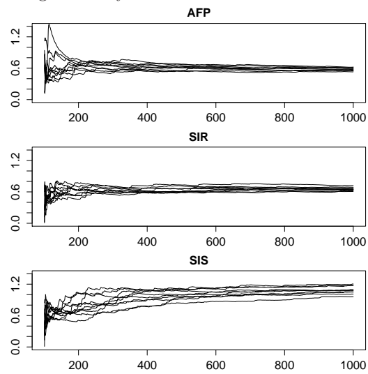
Figure 8: Comparison on weekly datasets of cumulative RMSEs between the true and the filtered log-volatility.
