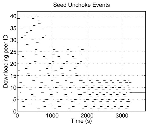
Figure 7: Duration of all unchokes (regular and optimistic) performed by a well-provisioned seed to each peer. Results for a single representative run. Peers 1 to 13 have a 20 kB/s upload limit, peers 14 to 27 have a 50 kB/s upload limit, and peers 28 to 40 have a 200 kB/s upload limit. The seed (peer 41) provides uniform service to all leechers.
