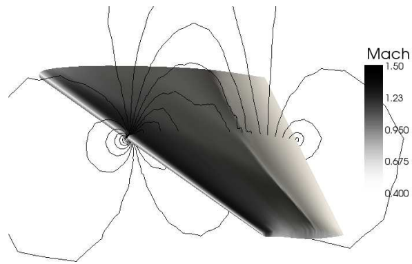
(b) M_\infty = 0.83
