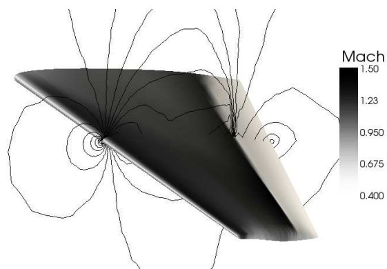
(c) M_\infty = 0.85
