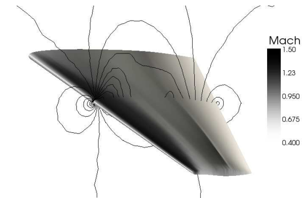
(a) M_\infty = 0.81
