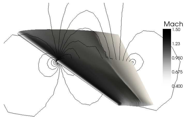
(b) M_\infty = 0.83
