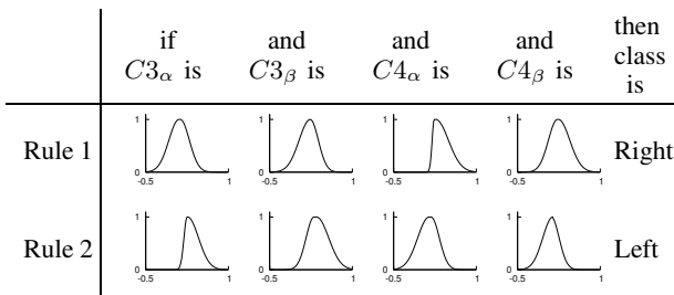
Fig. 1. Fuzzy rules automatically extracted by CFIS for subject 1.
