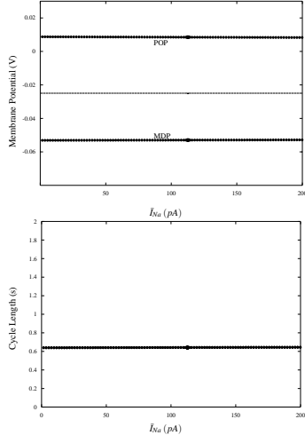
Fig. 4. Effects of changing current conductance \bar{I}_{Na} . Notations are similar to fig. 1.
