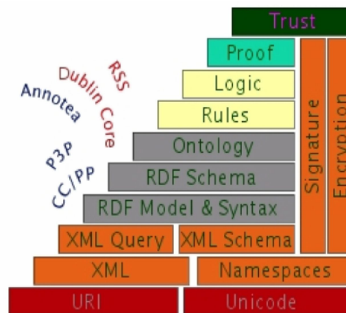
figure 1. The Layer Cake - from Tim Berners Lee.
