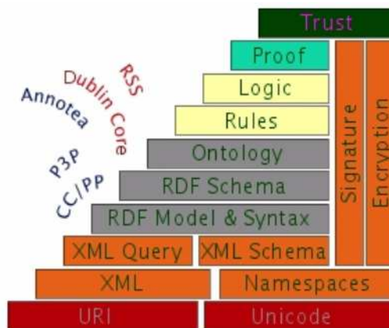
Figure 1: The Layer Cake - from Tim Berners Lee.
