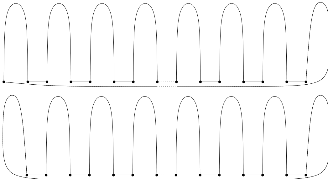
Figure 23: Two comb-like monotone locally convex polygons T_1 (top) and T_2 (bottom) with an odd and even number of vertices, respectively. Both polygons require \lfloor \frac{n}{2} \rfloor + 1 point guards in order to be guarded: one point guard is required per prong.
