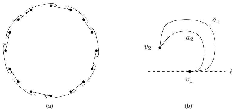
Figure 22: (a) A locally convex polygon with n vertices that requires n vertex or point guards in order to be guarded. (b) A non-convex polygon that cannot be guarded by vertex guards, and which requires an infinite number of point guards.
