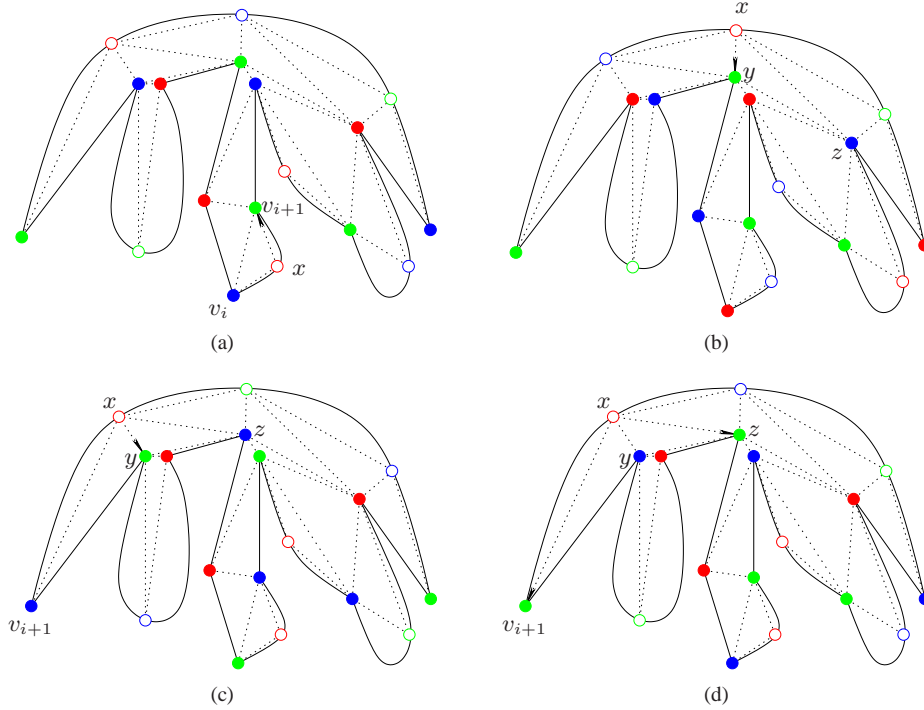
Figure 10: The three cases in the definition of the mapping f . Case (a): x is an auxiliary vertex in an empty room. Case (b): x is an auxiliary vertex in a non-empty room and is not the last auxiliary vertex added on the curvilinear arc. Cases (c) and (d): x is the last auxiliary vertex added on the curvilinear arc of a non-empty room (in (c) only one of its neighbors in P is green, whereas in (d) two of its neighbors in P are green).
