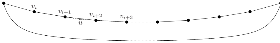
Figure 15: The crescent-like piecewise convex polygon C , that requires a guarding set of at least \lfloor \frac{n}{2} \rfloor vertex guards.
