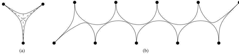
Figure 18: (a) A piecewise concave polygon P that cannot be guarded solely by vertex guards. Two consecutive edges of P have a common tangent at the common vertex and as a result the three vertices of P see only the points along the dashed segments. (b) A piecewise concave polygon P that requires 2n - 4 point guards in order to be guarded.
