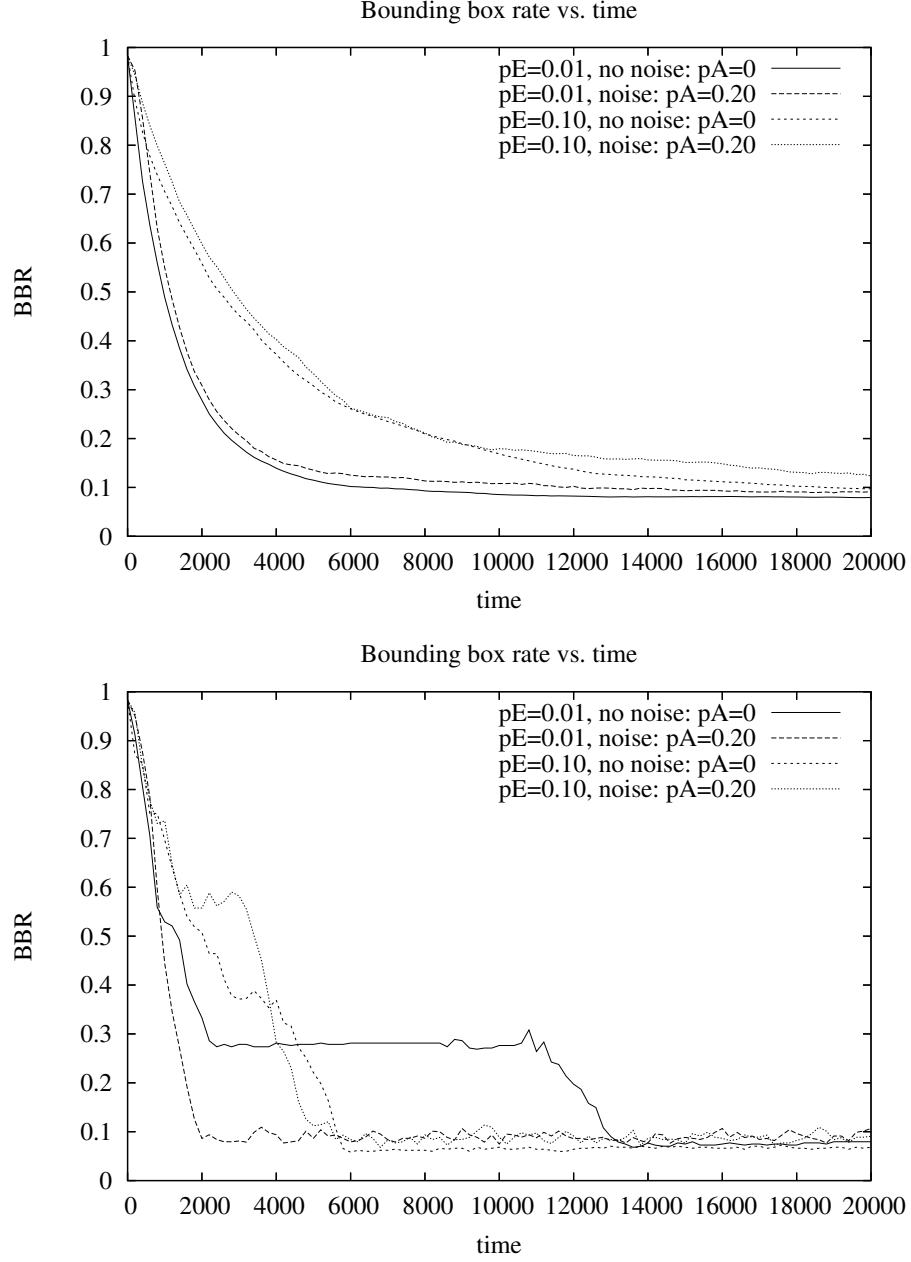
Figure 11: Evolution of the BBR as a function of time for a grid size (150, 100) , p_T = 1 , and different values of p_E and p_A . Average evolution for 100 samples (top) Example of a single sample evolution (bottom).
