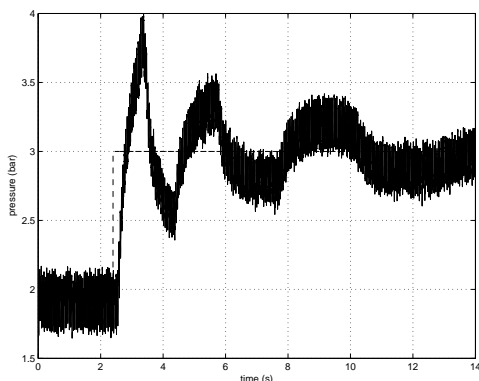
Fig. 3. Pressure evolution after set point changes from 2bar to 3bar for a = 10 , E = 30 , \hat{h} = 0 , (full line: measured pressure, dashed line: set point)
