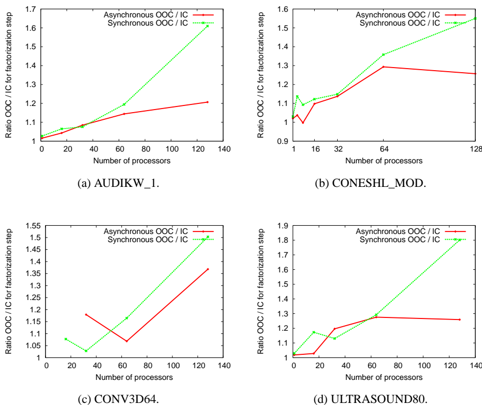
Figure 7: Execution times (normalized with respect to the in-core case) of the synchronous and asynchronous I/O schemes.
