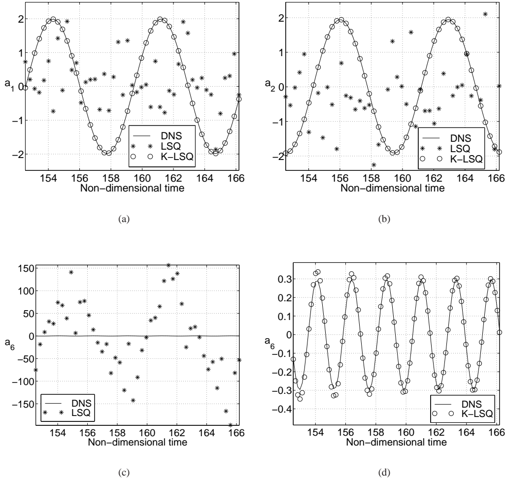
Figure 3: (a) and (b): POD modal coefficients a_1 and a_2 estimated with the K-LSQ and the LSQ approaches, compared to their exact values computed by projection of the DNS velocity fields. (c) coefficient a_6 , DNS and LSQ; (d) coefficient a_6 , DNS and K-LSQ. Note that in (c) and (d) different axis scales are used.
