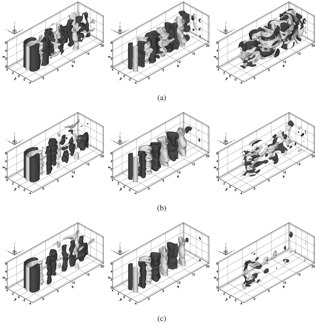
Figure 6: Isosurfaces of the velocity components u (left, grey = 0.5, dark grey = 1.0), v (center, grey = -0.25, dark grey = 0.25) and w (right, grey = -0.075, dark grey = 0.075) of a snapshot outside the database: (a) actual snapshot, (b) snapshot projected on the retained POD modes, (c) reconstructed snapshot using the K-LSE technique with the sensor configuration (b).
