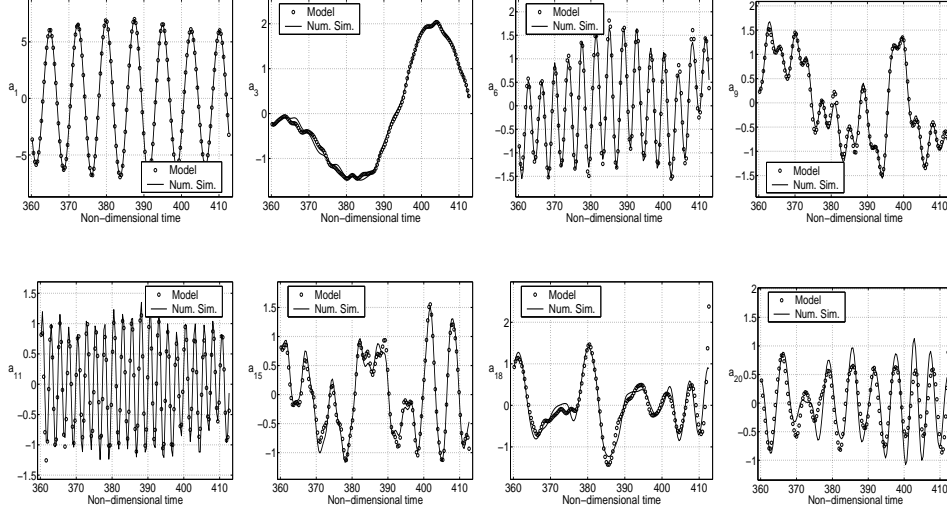
Figure 2: Three-dimensional flow: projection of the fully resolved Navier-Stokes simulations over the POD modes (continuous line) vs. the integration of the dynamical system inside the calibration interval, obtained retaining the first 20 POD modes (circles). Only 8 representative modal coefficients are shown here.
