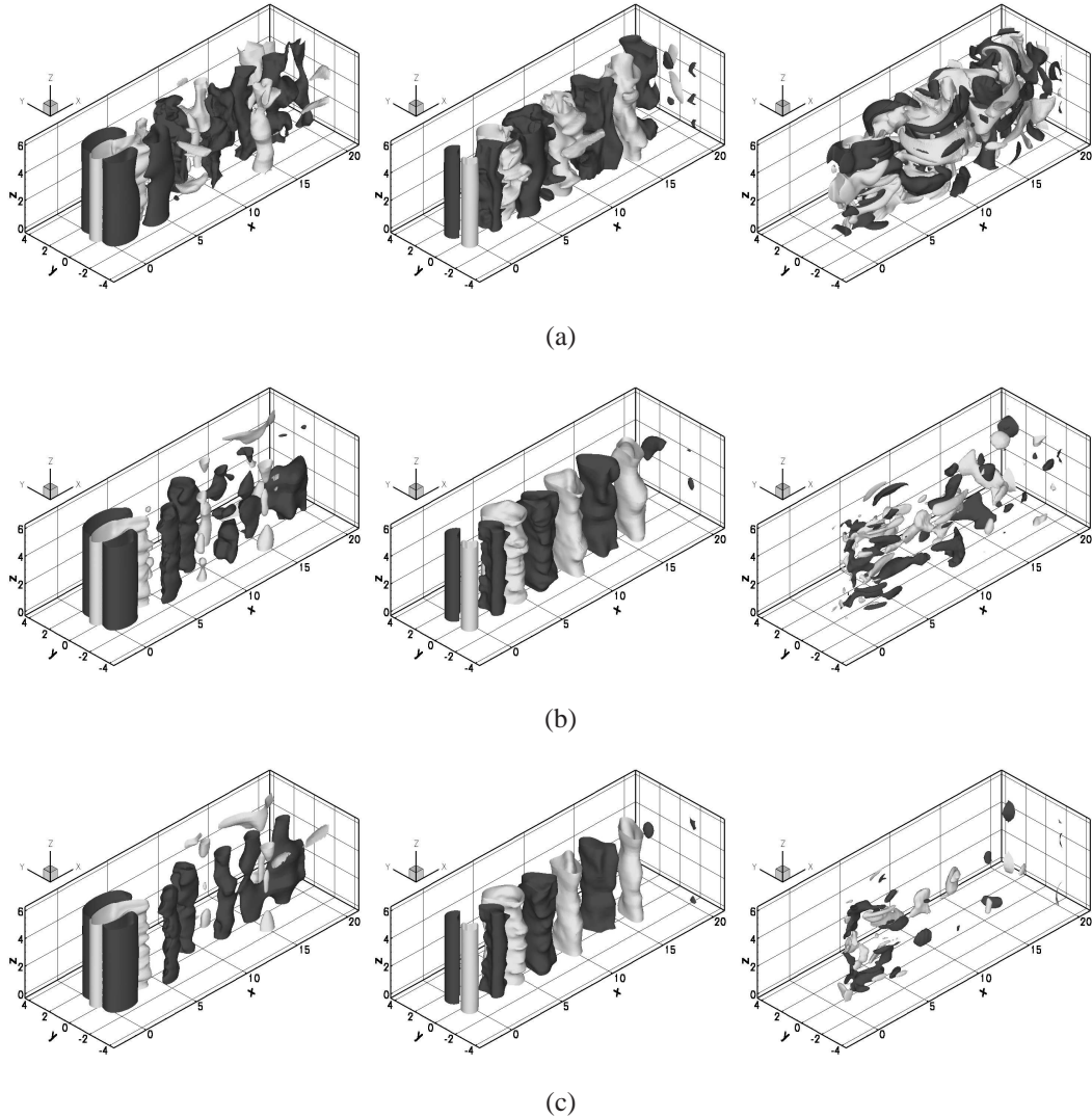
Figure 6: Isosurfaces of the velocity components u (left, grey = 0.5, dark grey = 1.0), v (center, grey = -0.25, dark grey = 0.25) and w (right, grey = -0.075, dark grey = 0.075) of a snapshot outside the database: (a) actual snapshot, (b) snapshot projected on the retained POD modes, (c) reconstructed snapshot using the K-LSE technique with the sensor configuration (b).
