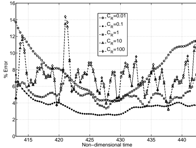
Figure 4: Relative percent error in the reconstruction of the U component projected on the retained POD modes as a function of time, when varying C_R .
