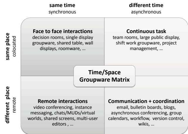
Figure 1. CSCW Matrix
