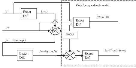
Figure 3. Observer scheme
