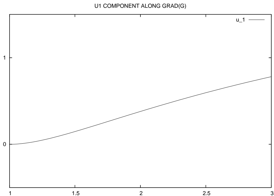
Figure 5: Concurrent minimization of the criteria J_A and J_B in the case of a nonlinear equality constraint; variation with A of the optimization variable u_1 , component of the state perturbation along the constraint gradient.
