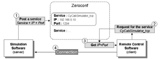
Figure 3: Zero Configuration Networking
