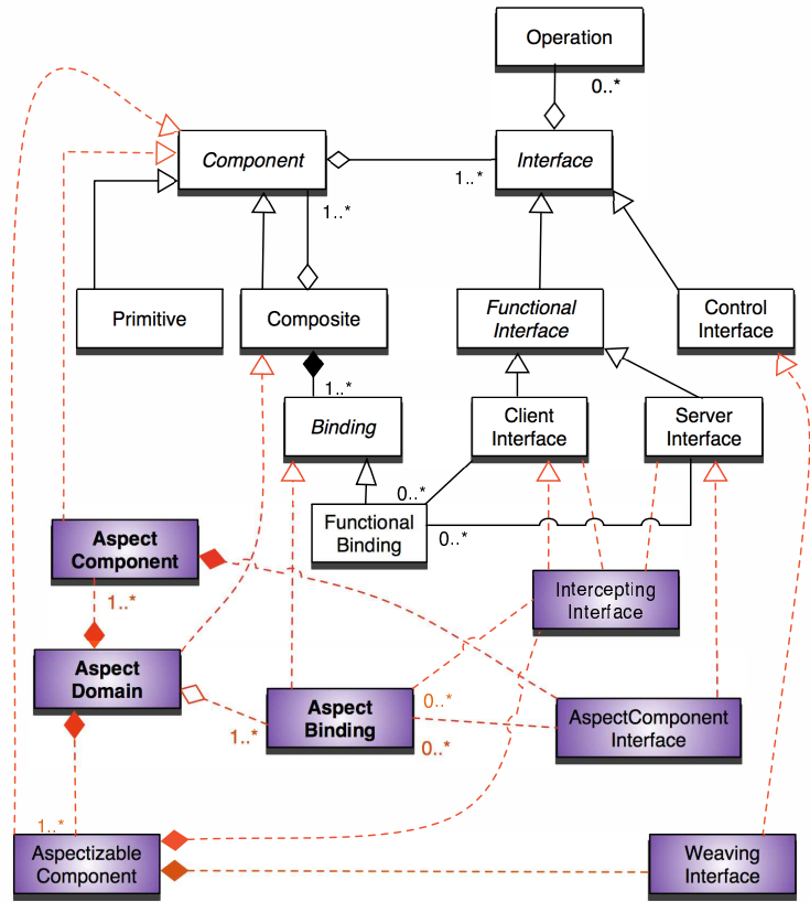
Fig. 5. FAC metamodel
