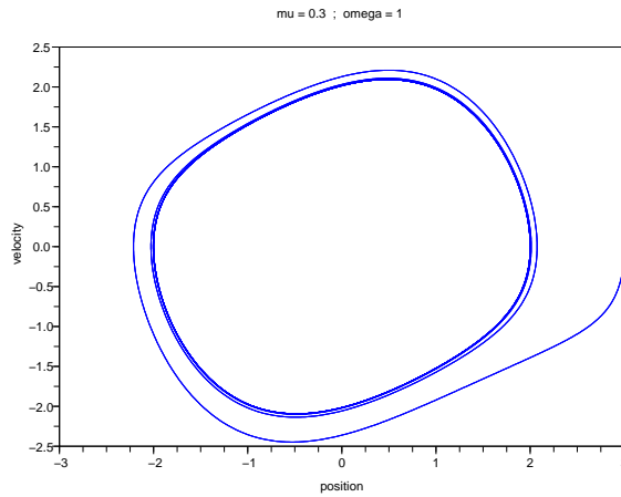
Figure 1: Limit cycle of the van der Pol oscillator. Here \mu = 0.3 and \omega_0 = 1 .
