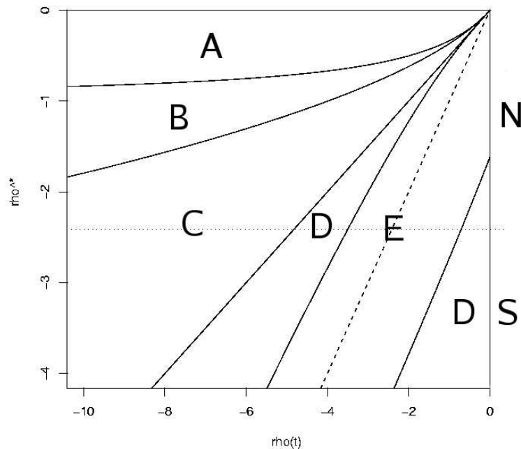
Figure 1: Comparison of the asymptotic bias and variances
