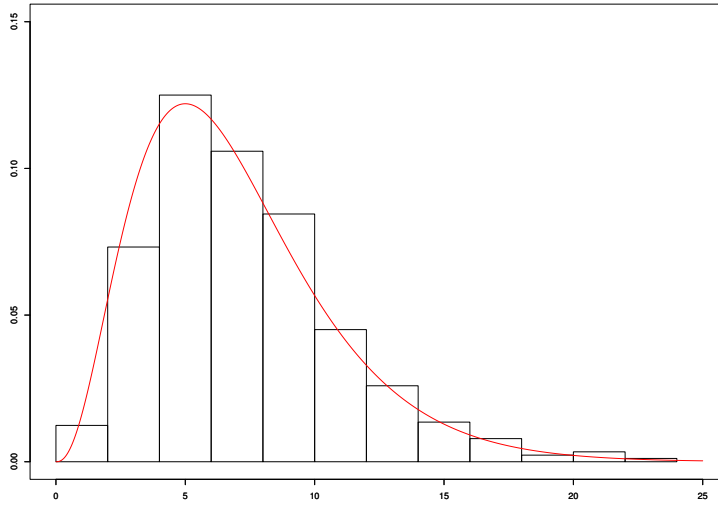
Figure 2: Histogram of the \chi^2 distances between the rescaled log-spacings and the standard exponential distribution. The theoretical density of the corresponding \chi^2 distribution is superimposed.
