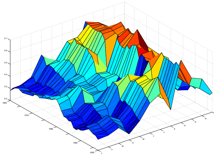
Figure 3: Conditional Zipf estimator \tilde{\gamma}_n(t, \mu^Z) of the tail index computed on the real dataset. Two covariates are available: The year ranging from 1969 to 2005 and the day ranging from 1 to 365. For the sake of readability, only the first letter of the corresponding month is represented.
