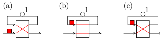
Figure 2: Optical memory cell: (a) writing information (b) circulation information (c) reading information.
