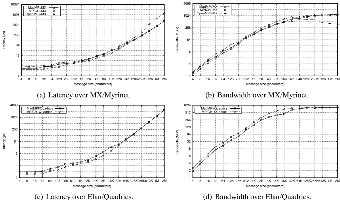
Figure 2: Raw point-to-point ping-pong.
