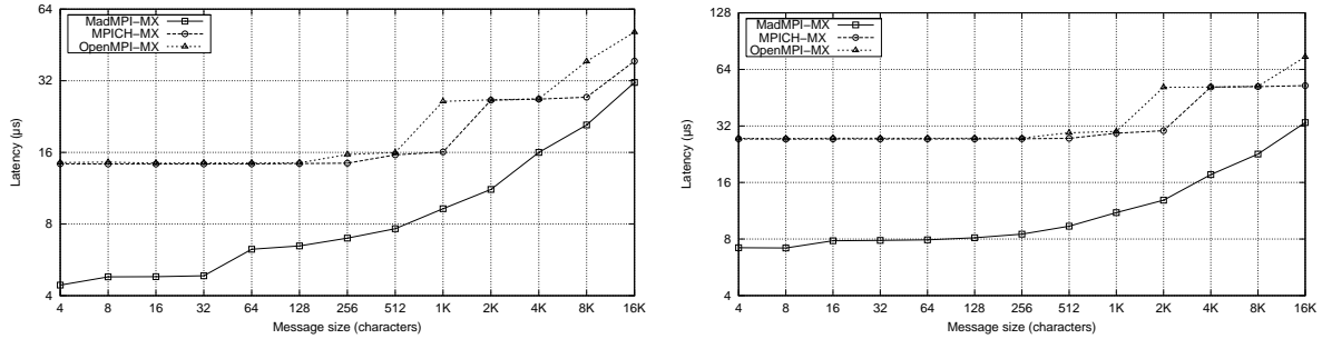
(a) 8-segments ping-pong - Latency over MX/Myrinet. (b) 16-segments ping-pong - Latency over MX/Myrinet.
