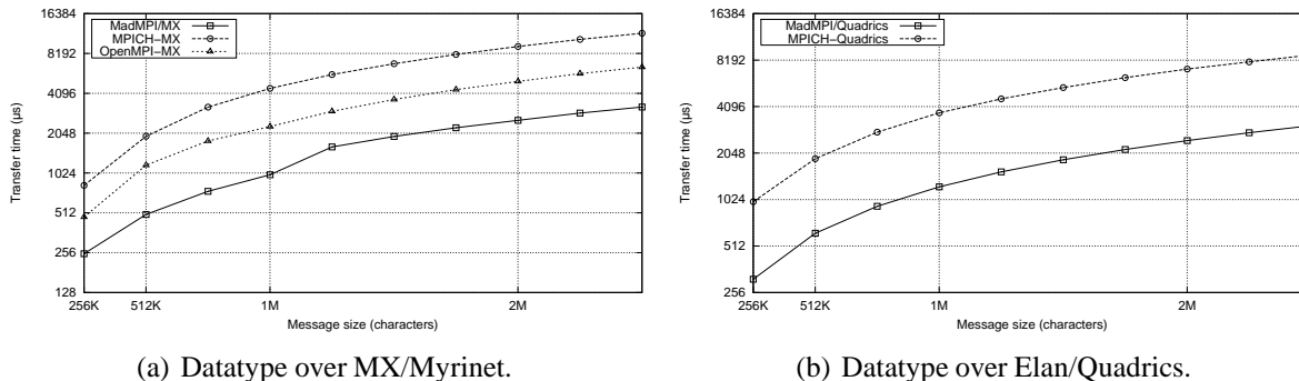
Figure 4: Indexed datatype.
