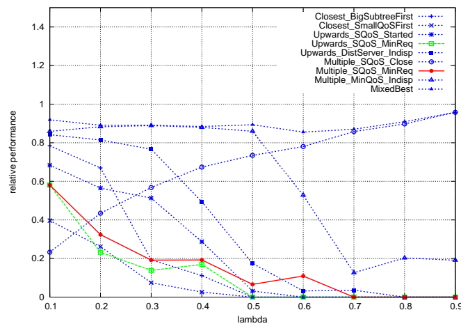
Figure 26: Impact of QoS constraints in big trees, qos = \text{height} + 1 \rightarrow no QoS.
