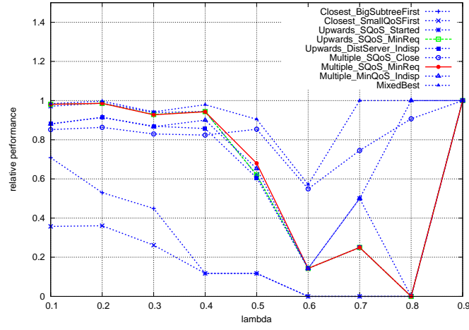
Figure 21: Impact of QoS constraints in small trees, \text{qos} \in \{1, 2\} .
