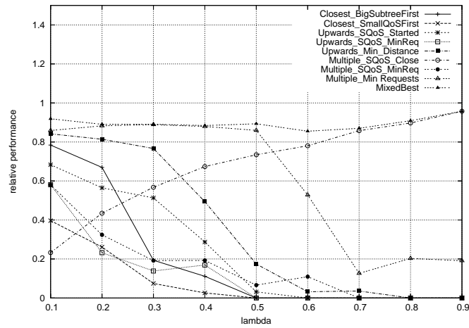
Figure 14: Relative performance for big trees, \text{qos} = \text{height} + 1 \rightarrow \text{no QoS} .
