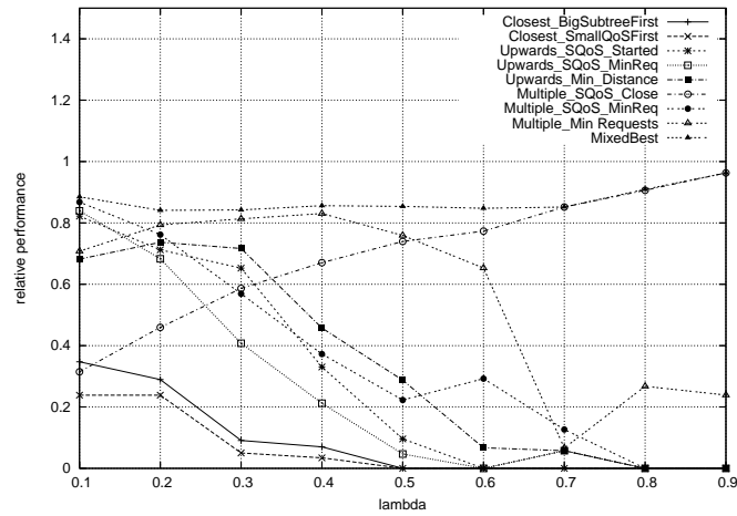
Figure 13: Relative performance for big trees, \text{average\_qos} = \text{height}/2 .
