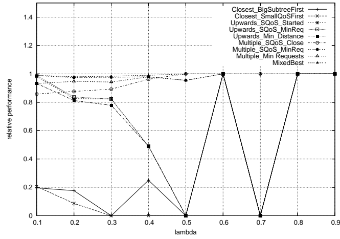
Figure 12: Relative performance for big trees, \text{qos} \in \{1, 2\} .
