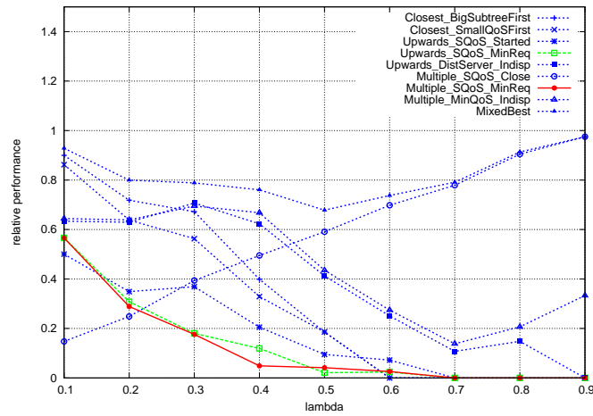
Figure 23: Impact of QoS constraints in small trees, \text{qos} = \text{height} + 1 \rightarrow \text{no QoS} .
