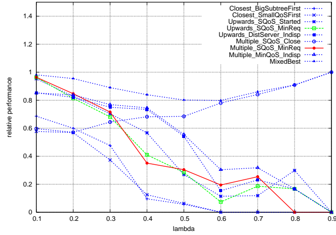
Figure 22: Impact of QoS constraints in small trees, \text{qos} = \text{average\_qos} = \text{height}/2 .
