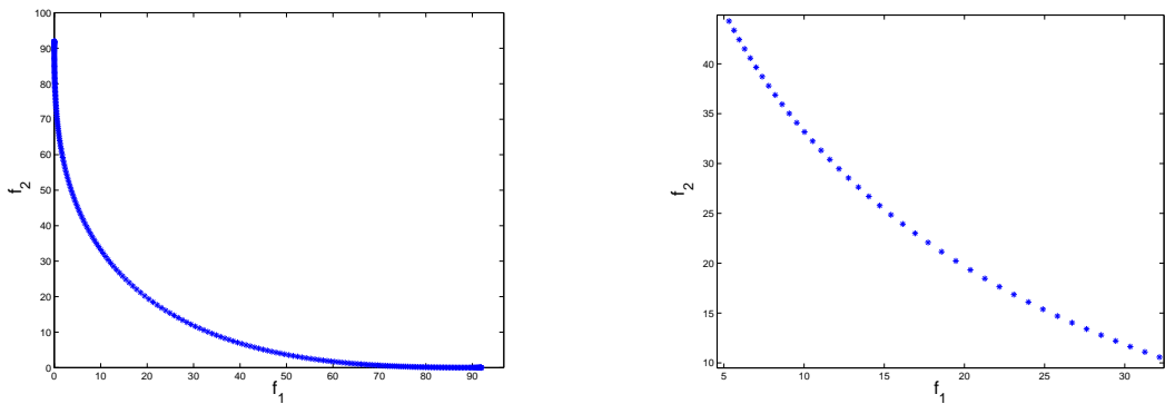
Figure 4: Result of the continuation method with step size control on MOP (17) for n = 20 in image space: all solutions (left) and zoom (right).
