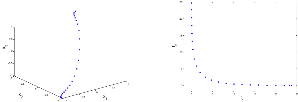
Figure 3: Result of the continuation method with step size control on MOP (17) for n = 3 in parameter space (left) and image space (right).
