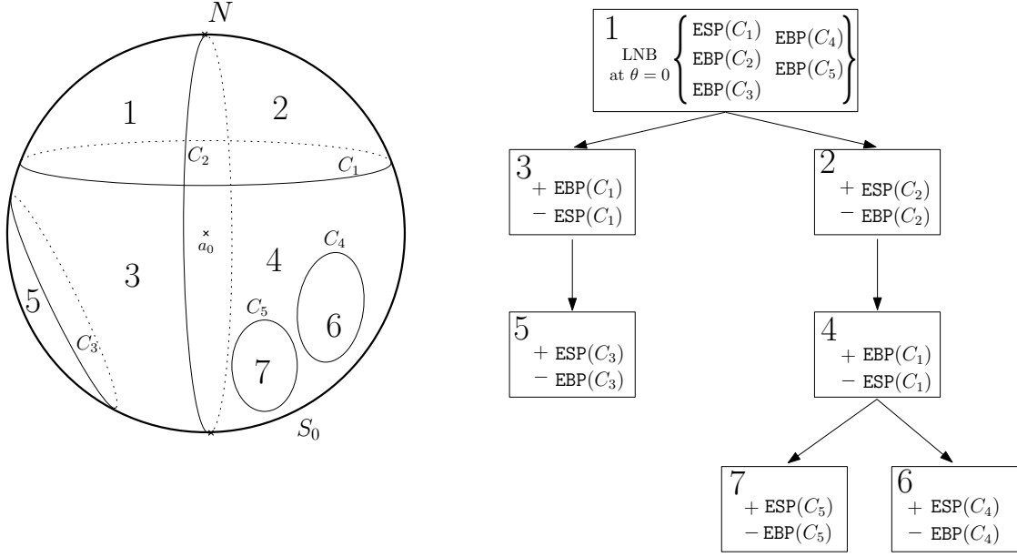
Figure 17 Implicit encoding of covering balls. Circle C_1 is a north threaded circle and C_2 a bipolar one, while C_3, C_4 and C_5 are normal ones. Faces of the arrangement depicted on the left are identified using numbers from 1 to 7. Notice that node associated to face 2 reflects the modification of LNB induced by bipolar circle C_2 .
