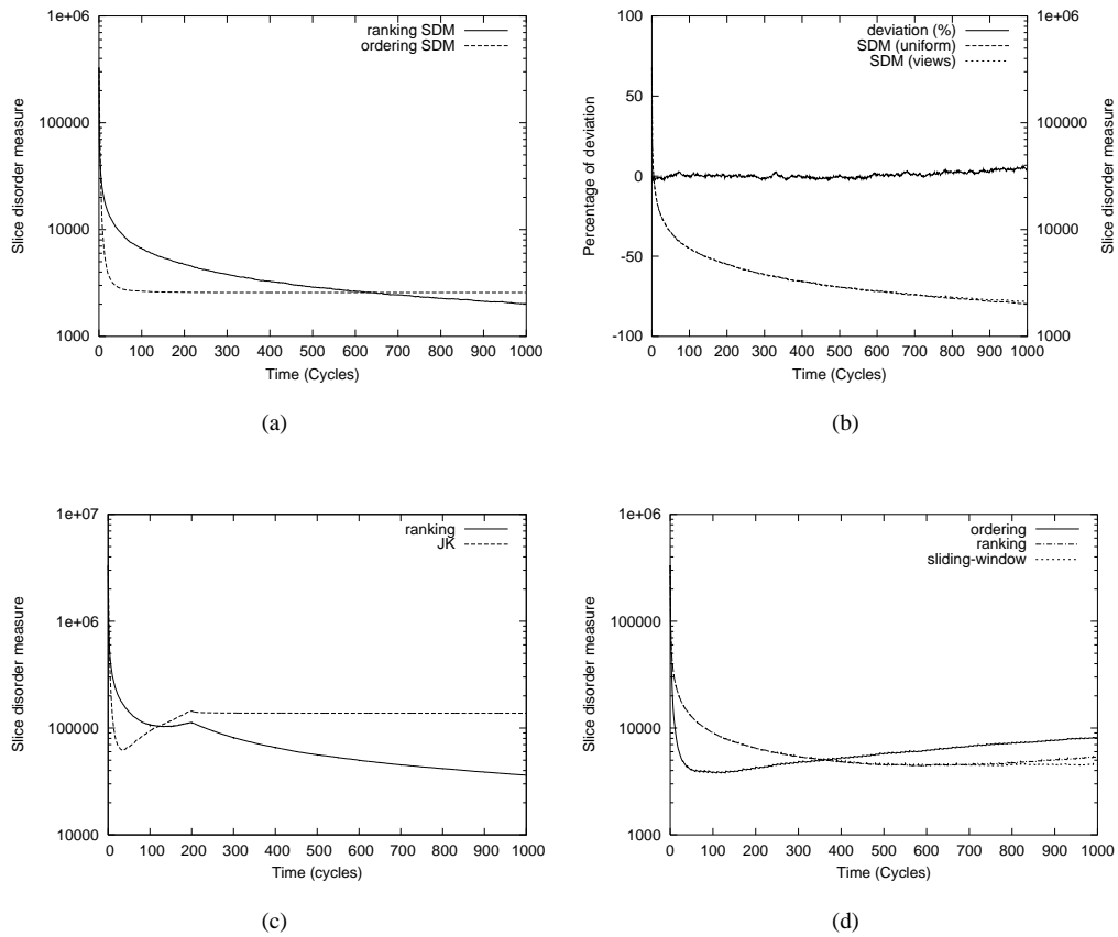
Figure 6: (a) Comparing performance of the ordering algorithm and the ranking algorithm (static case). (b) Comparing the ranking algorithm on top of a uniform drawing or a Cyclon-like protocol. (c) Effect of dynamics burst on the convergence of the ordering algorithm and the ranking algorithm. (d) Effect of a low and regular churn on the convergence of the ordering algorithm and the ranking algorithm.
