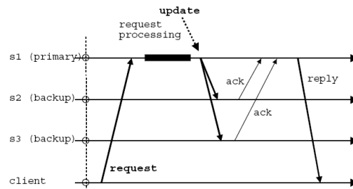
Figure 6: Primary-backup replication
