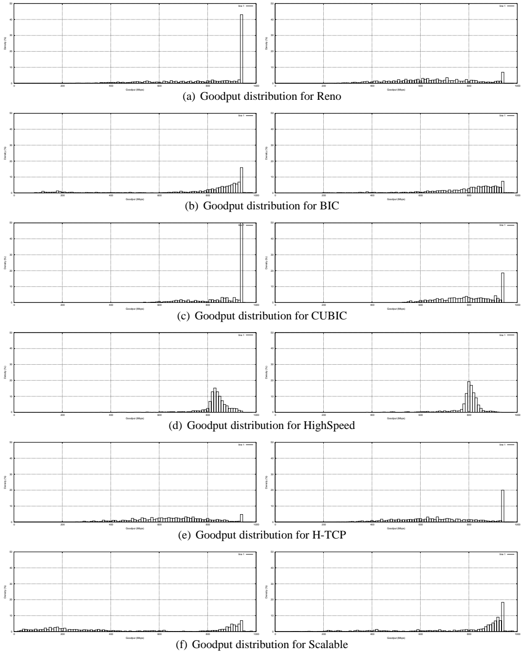
Figure 20: Examples of Goodput distribution for 11.5 ms RTT when 12 nodes are active, in AIST-GtrcNET-10
