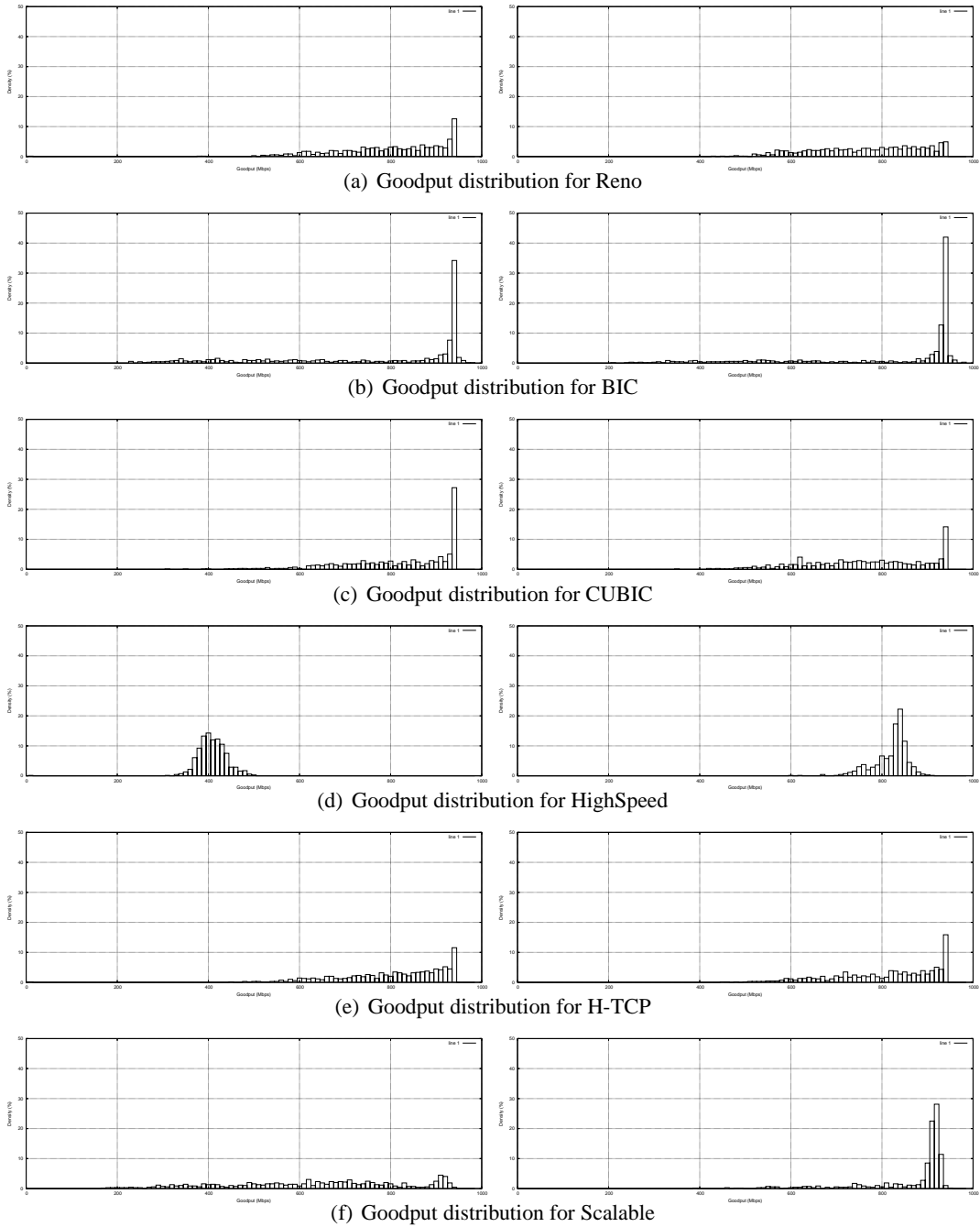
Figure 19: Examples of Goodput distribution for 0 ms RTT when 12 nodes are active, in AIST-GtrcNET-10
