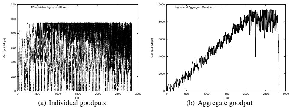
Figure 13: HighSpeed in AIST-GtrcNET-10 with 100 ms RTT
