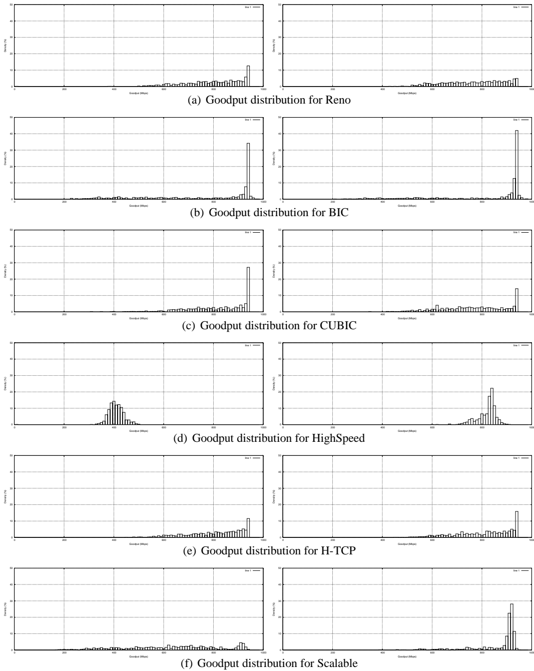
Figure 19: Examples of Goodput distribution for 0 ms RTT when 12 nodes are active, in AIST-GtrcNET-10
