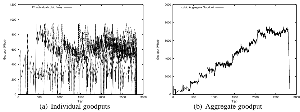
Figure 12: CUBIC in AIST-GtrcNET-10 with 100 ms RTT
