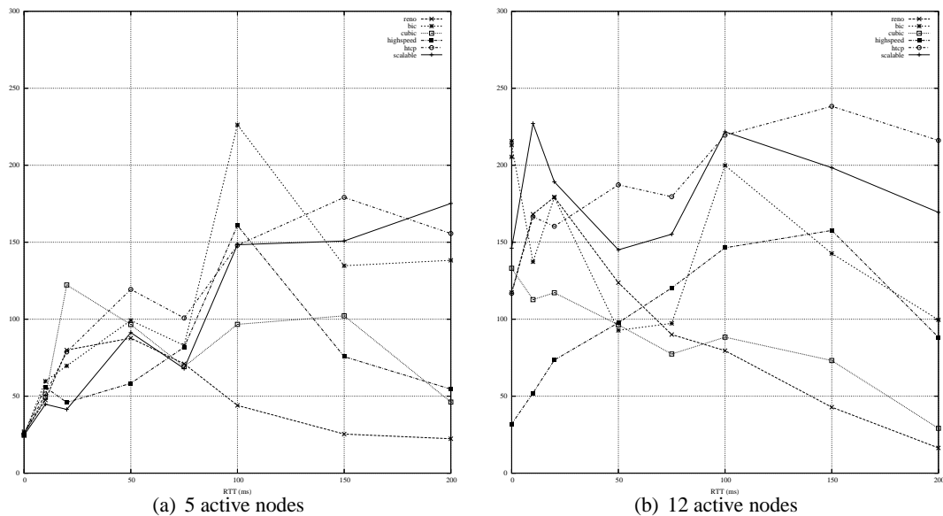
Figure 18: Mean of goodputs' standard deviation for TCP variants when 5 or 12 nodes are actives in AIST-GtrcNET-10
