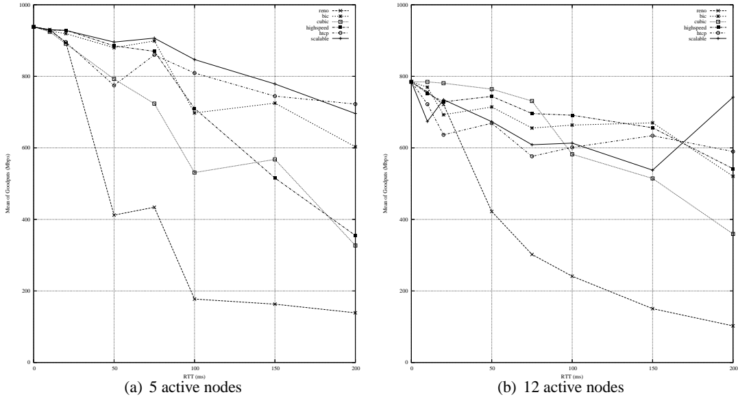
Figure 16: Mean goodputs for TCP variants when 5 or 12 nodes are active in AIST-GtrcNET-10
