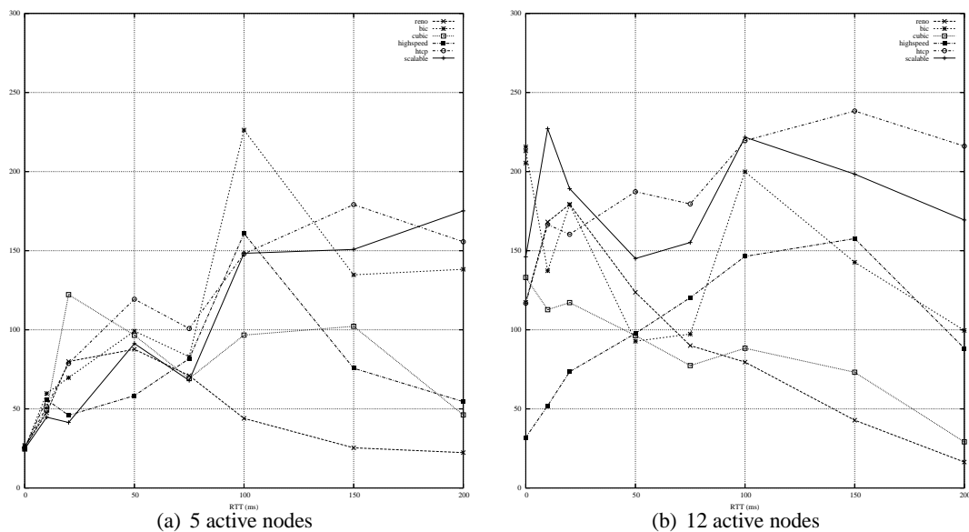
Figure 18: Mean of goodputs' standard deviation for TCP variants when 5 or 12 nodes are active in AIST-GtrcNET-10
