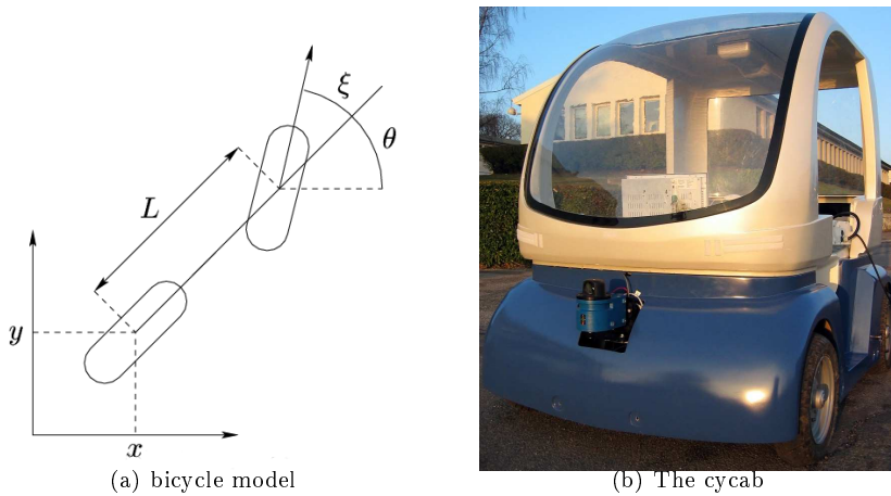
Figure 3 The car-like vehicle. \mathcal{A} .
