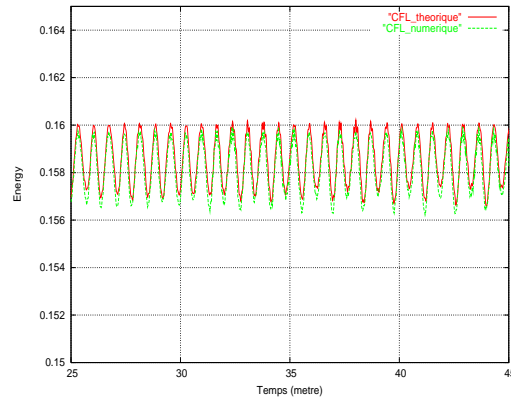
(b) GD- \mathbb{P}_1
