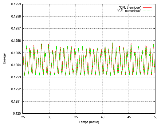
(c) GD- \mathbb{P}_2
