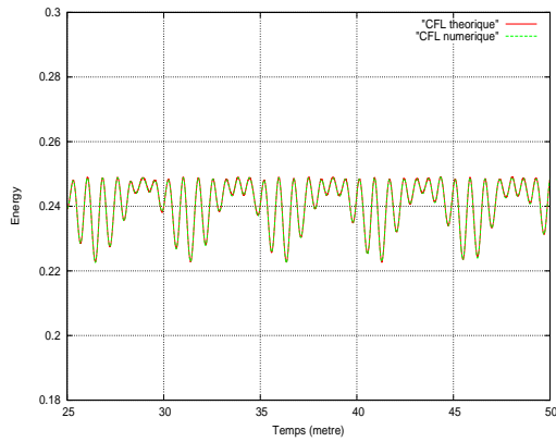
(a) GD- \mathbb{P}_0
