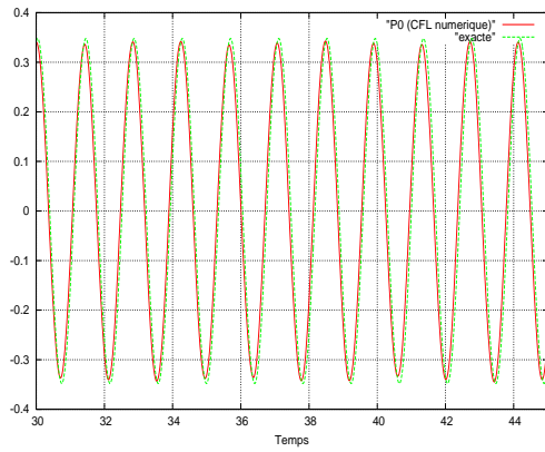
(a) Schéma GD- \mathbb{P}_0
