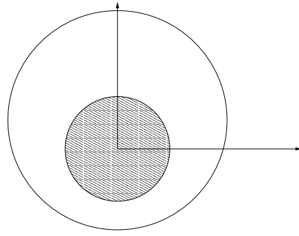
Figure 2. Computational domain for problem (31). \Gamma_1 is the inner circle of center (0, 0) and radius r = 1 , \Gamma_2 is the outer circle (center (0, 0.5) , radius r = 3 ).
