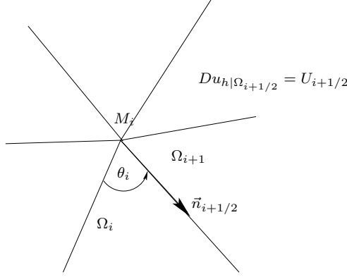
Figure 1. Illustration of the angular sectors \Omega_i , \theta_i and the vectors \vec{n}_{i+1/2} that are needed in numerical Hamiltonian definitions.
