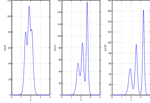
Fig. 1. A 3-soliton at three successive times 0, t_1 , t_2
