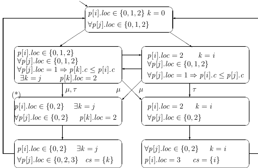
Fig. 5 A PDT for Fischer's protocol for N processes.
