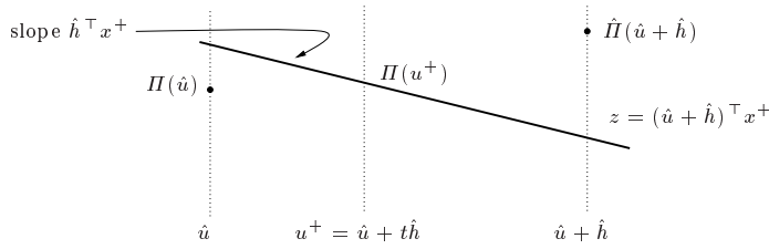
Fig. 7.1 The new linearization passes under \hat{\Pi}(\hat{u} + \hat{h})
