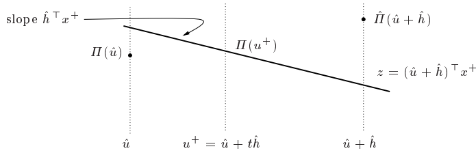
Fig. 7.1 The new linearization passes under \hat{\Pi}(\hat{u} + \hat{h})
