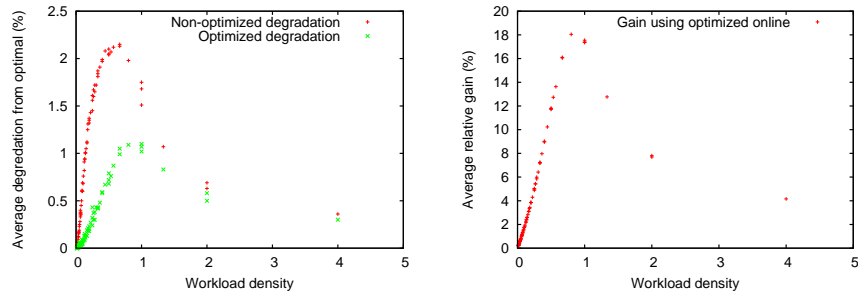
(a) Max-stretch degradation from optimal of both versions of the online heuristic (b) Sum-stretch gain of the optimized version, relative to the non-optimized version
