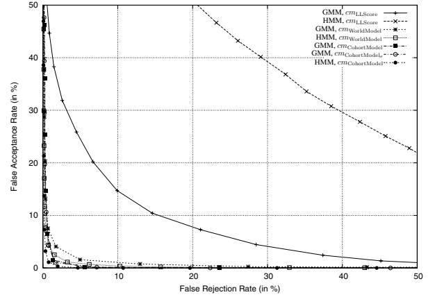
Figure 2. ROC curves of the HMM and the GMM based system on the unskillfully forged test set.
