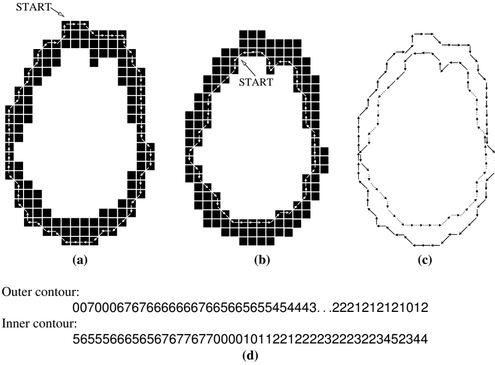
Figure 1. Extraction of chain-code from an off-line image by contour tracing; (a) outer contour tracing, (b) inner contour tracing, (c) contour profile, (d) resulting chain-coded descriptor strings of the character.
