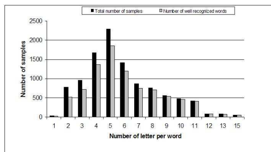
Figure 4. Evaluation of the robustness of the system according to the number of letters per word
