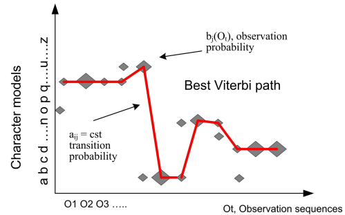
Figure 2. Recognition trellis and Dynamic programming for the french word "quand"
