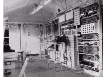
Colossus I (1943)
