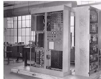
EDVAC (1945)
