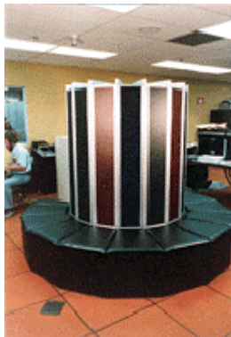
CRAY I (1976)
