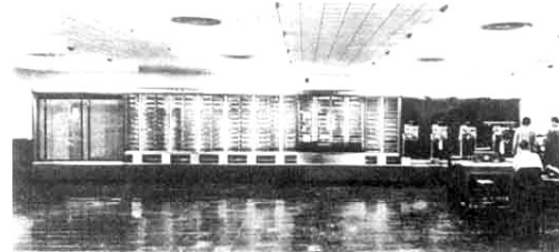
Harvard MARK 1 (1943)
