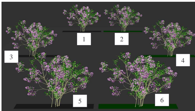
Fig.6 View-dependant simplification
